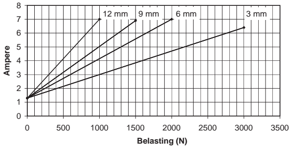
LA30 24V S-motor stroom versus belasting
