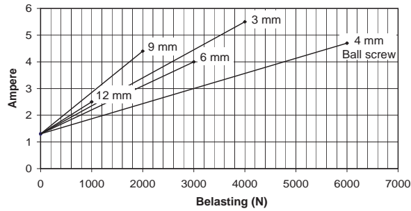
LA30 12V motor stroom versus belasting
